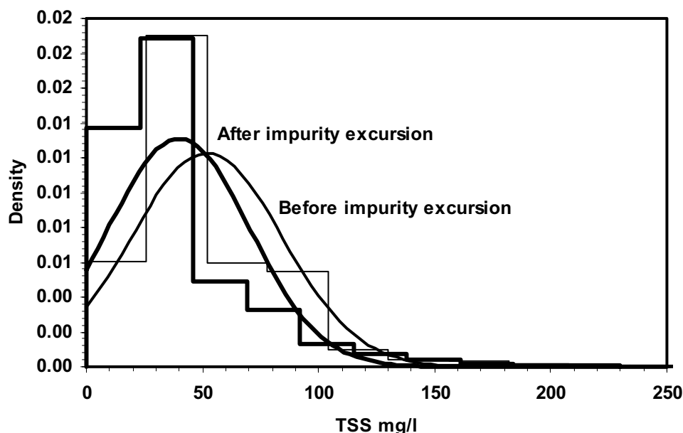
Figure 5: Frequency distributions of total suspended solids (TSS) entering SX.
