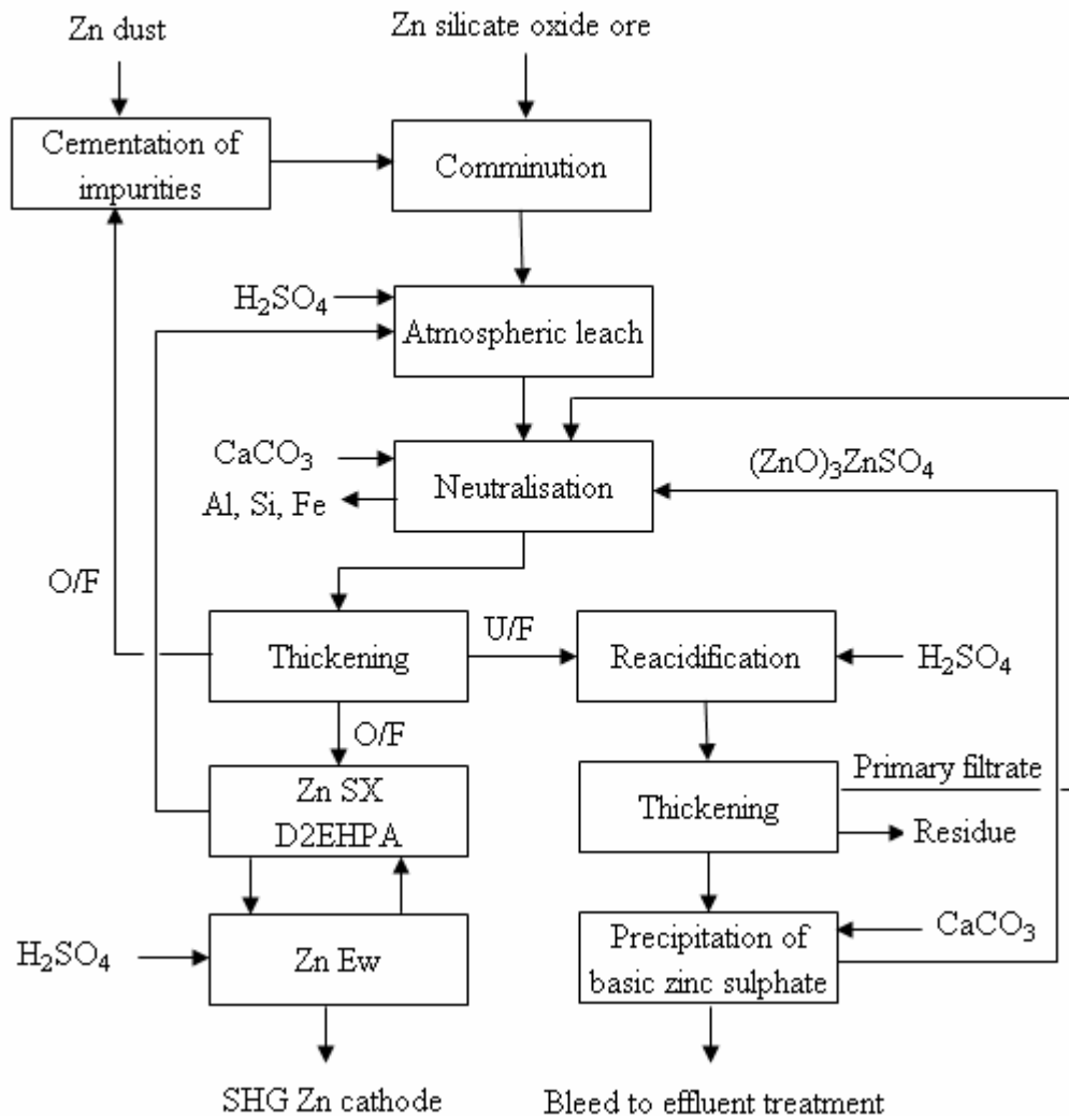
Figure 2: Simplified process flowsheet of the Skorpion Zinc refinery.
