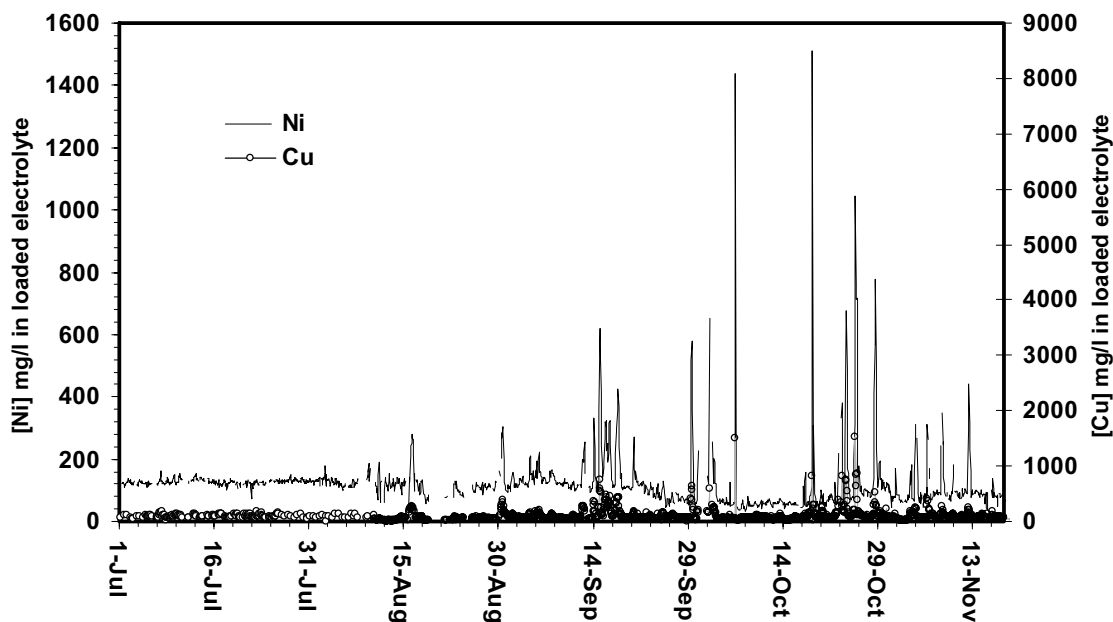
Figure 4: Evolution of impurities concentrations in loaded electrolyte (1 July -18 November 2006).
