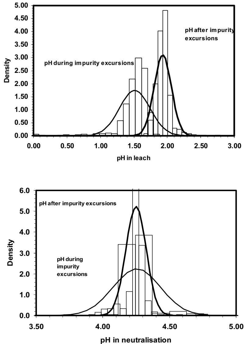
Figure 7: Frequency distributions of pH a) in last leach tank b) in neutralisation.
