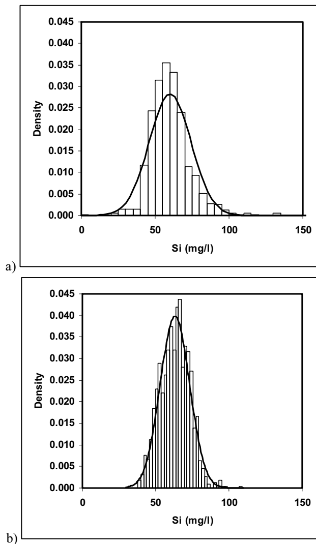
Figure 6: Frequency distributions of Si in PLS a) during impurity excursions b) after impurity excursions.
