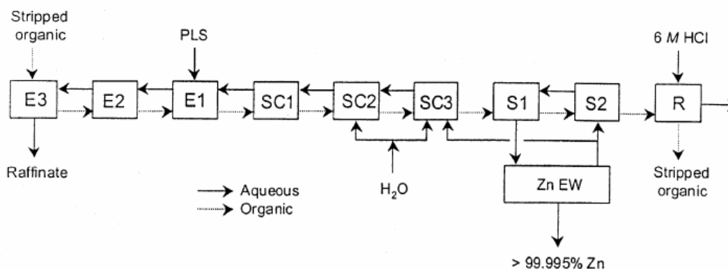
Figure 3: Schematic representation Skorpion SX circuit.
