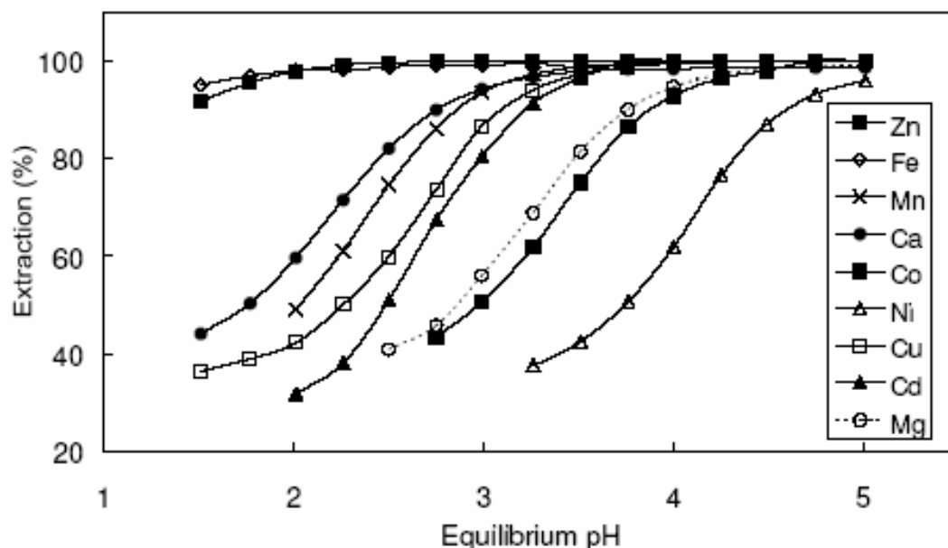
Figure 1: Effect of pH on the selectivity of extraction of base-metal cations in the Skorpion Zinc system. Conditions: 40 vol.% D2EHPA in Escaid 100, 40 °C 30g/l Zn in feed (4).
