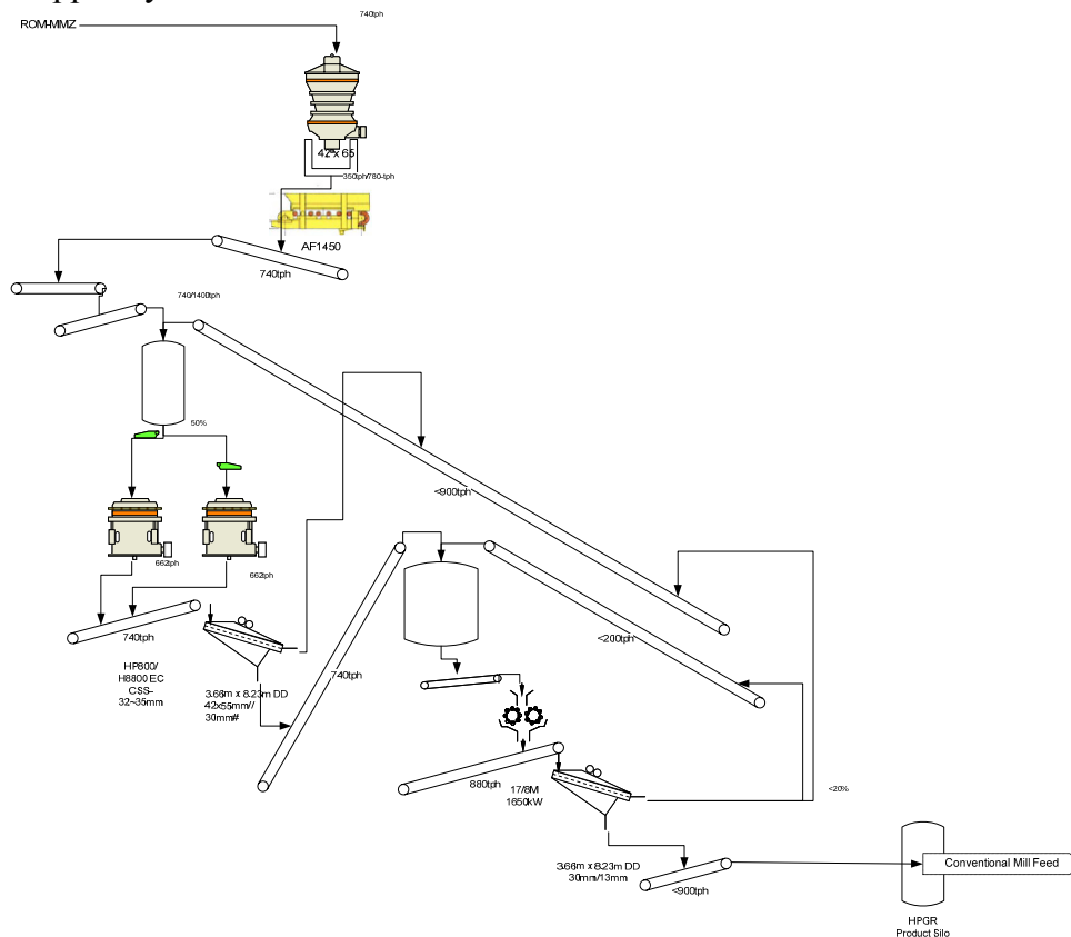
Figure 6 - HPGR Tertiary Crushing
