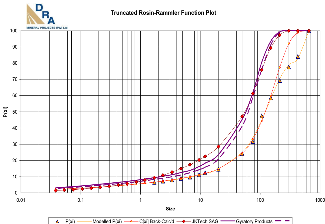
Figure 3 - Measured typical ROM & Estimated Minus 200mm Distributions
