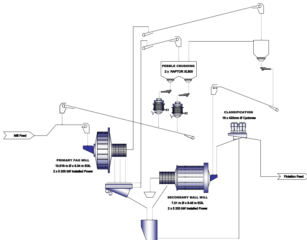
Figure 7 : Proposed Milling Circuit for Nkomati Main MMZ Plant
