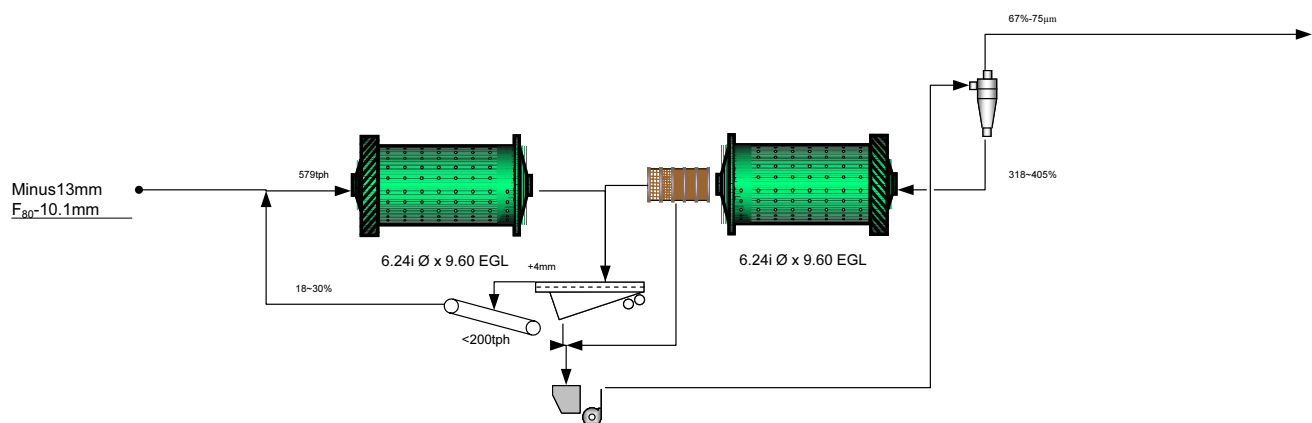
Figure 5 - Proposed Conventional Milling Circuit
