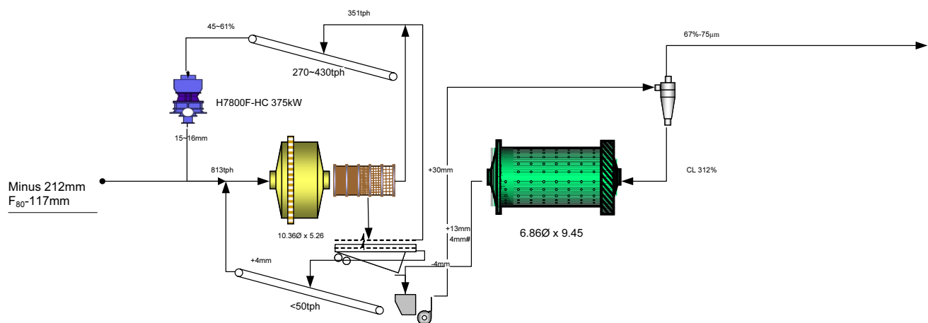
Figure 4 - SABC Milling Circuit
